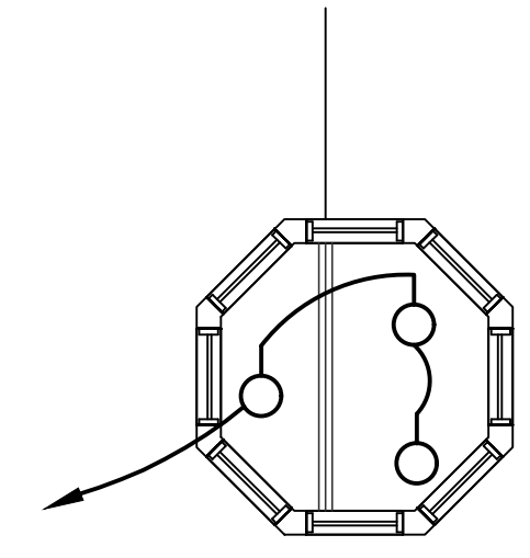
2 CUPOLA PLAN (LIGHT WELL) SCALE: 1/4"=1'-0"
